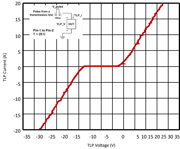
Fig 3. TLP Measurement
