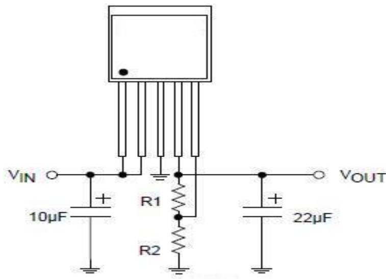
MIC29302WU(MS)典型应用图
