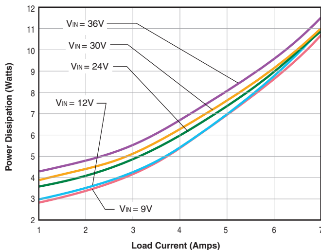
UQQ-15/7-Q12P Power Dissipation vs. Load Current @ 25°C
