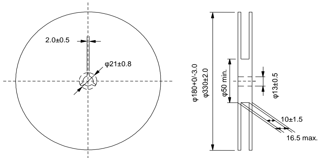
Fig.3 Taping Diagram
