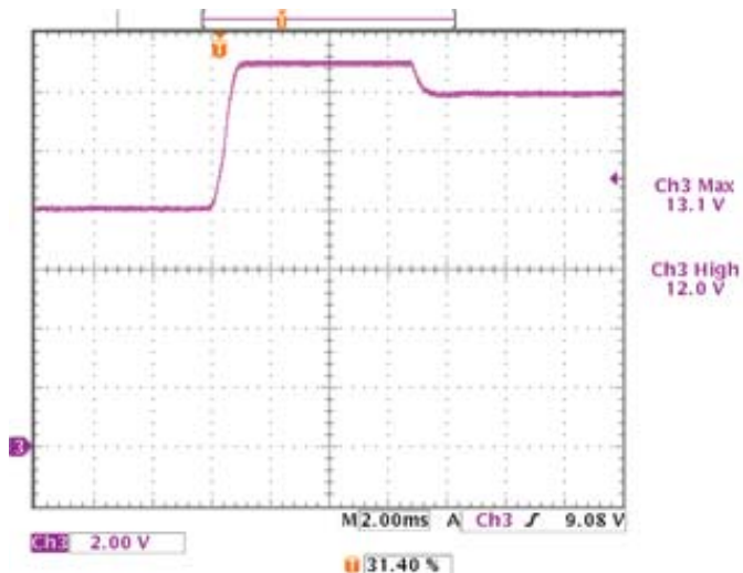
Typical Startup Waveform with a 8V bias voltage
