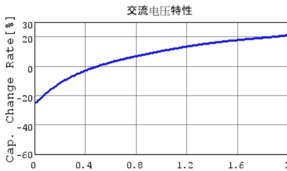
GRM022R61A102KE19 C-AC Voltage capchange, DC
