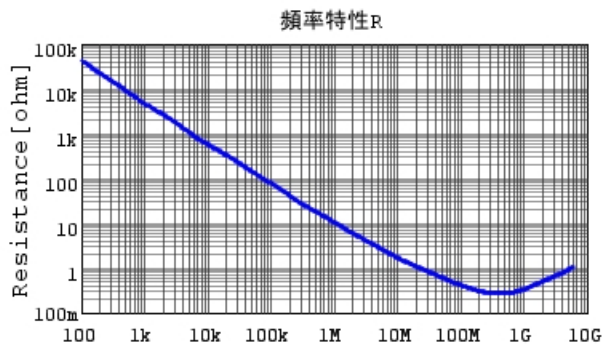
GRM022R61A102KE19 R DCOV, 25degC
