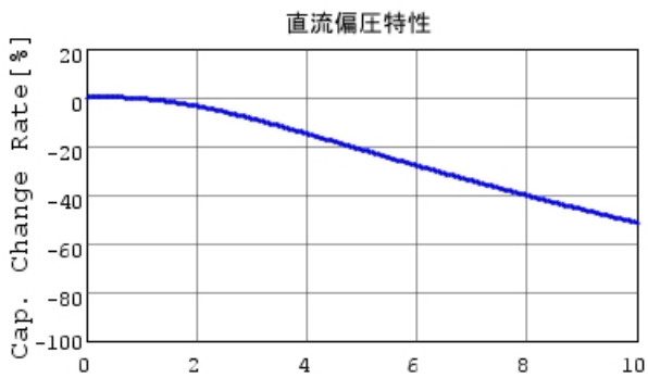
GRM022R61A102KE19 C-DC bias capchange, 25.0c
