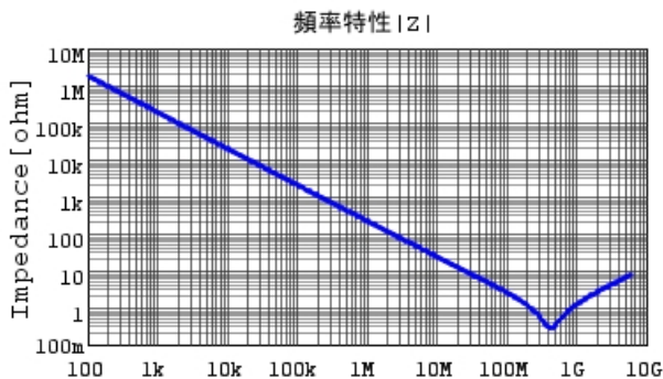
GRM022R61A102KE19 |Z| DCOV, 25degC
