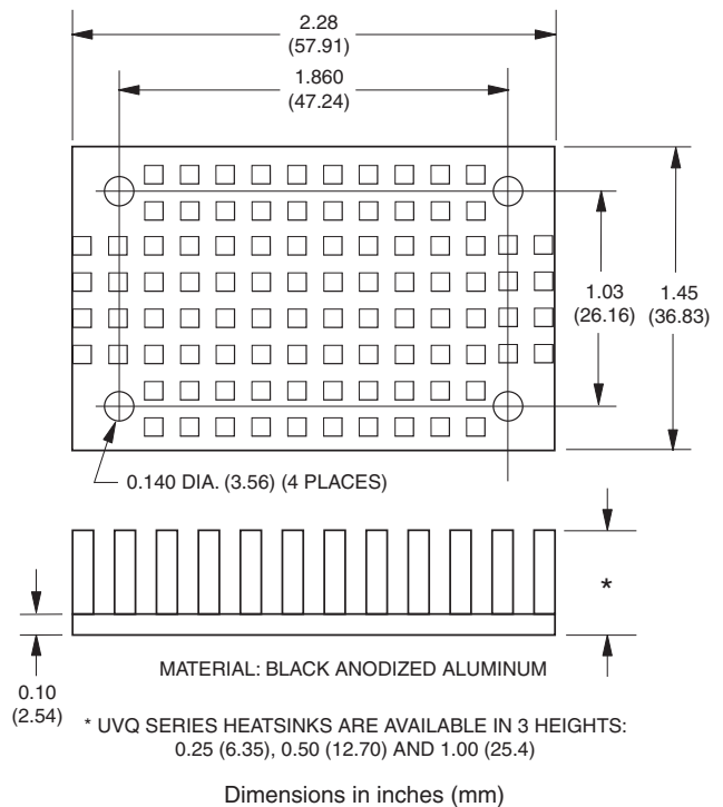
Dimensions in inches (mm)
