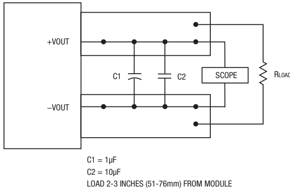
Figure 3. Measuring Output Ripple and Noise (PAR)
