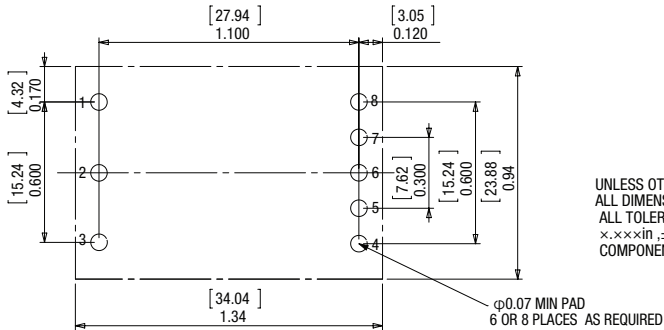
RECOMMEND PCB FOOTPRINT
