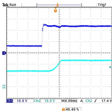
Pre-biased output voltage added connecting an external 680µF to the output ( V_{in}=24V , I_{out}=0A , +25^\circ C )
