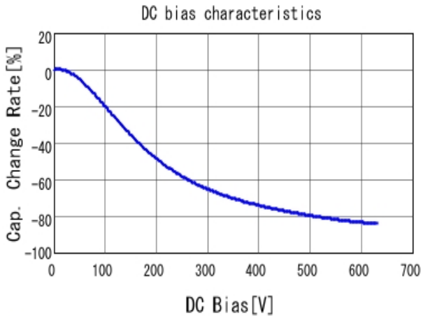
■ RDER72J474MUB1H03B C-DC bias capchange, 25.0degC, AC1
