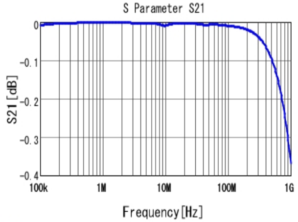
■ RDER72J474MUB1H03B S21 DCOV, 25degC
