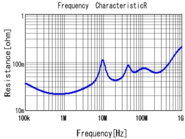
■ RDER72J474MUB1H03B R DCOV, 25degC
