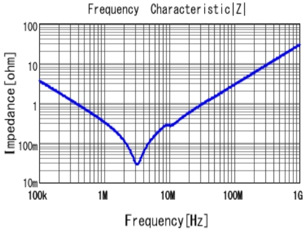
■ RDER72J474MUB1H03B |Z| DCOV, 25degC
