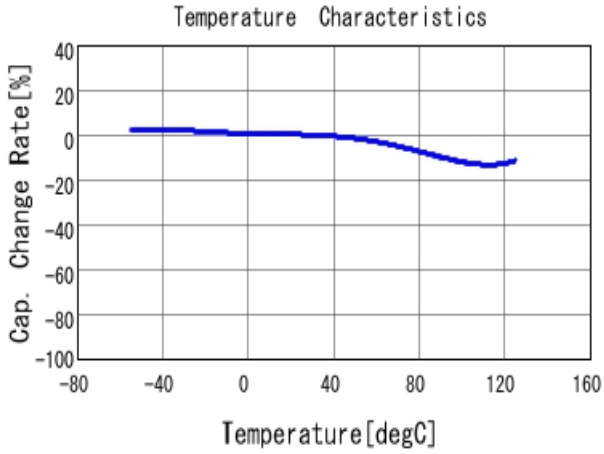
■ RDER72J474MUB1H03B C-Temp. capchange, DCOV, AC1Vrms
