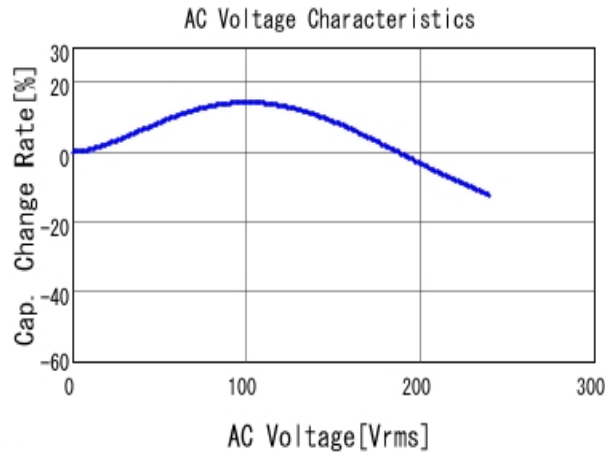
■ RDER72J474MUB1H03B C-AC Voltage capchange, DCOV, 25.0
