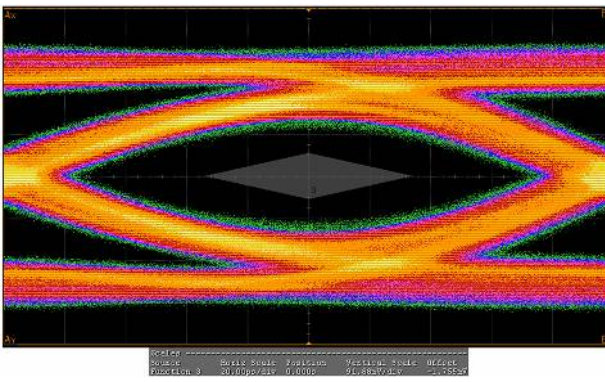
Signal Integrity USB3.0 0ohm
