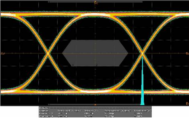
Signal Integrity HDMI 1080P 48bit 0ohm
