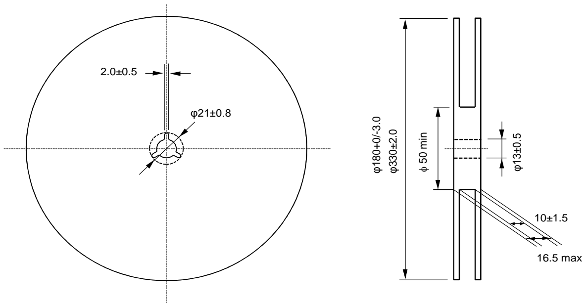
Fig3 Taping Diagram
