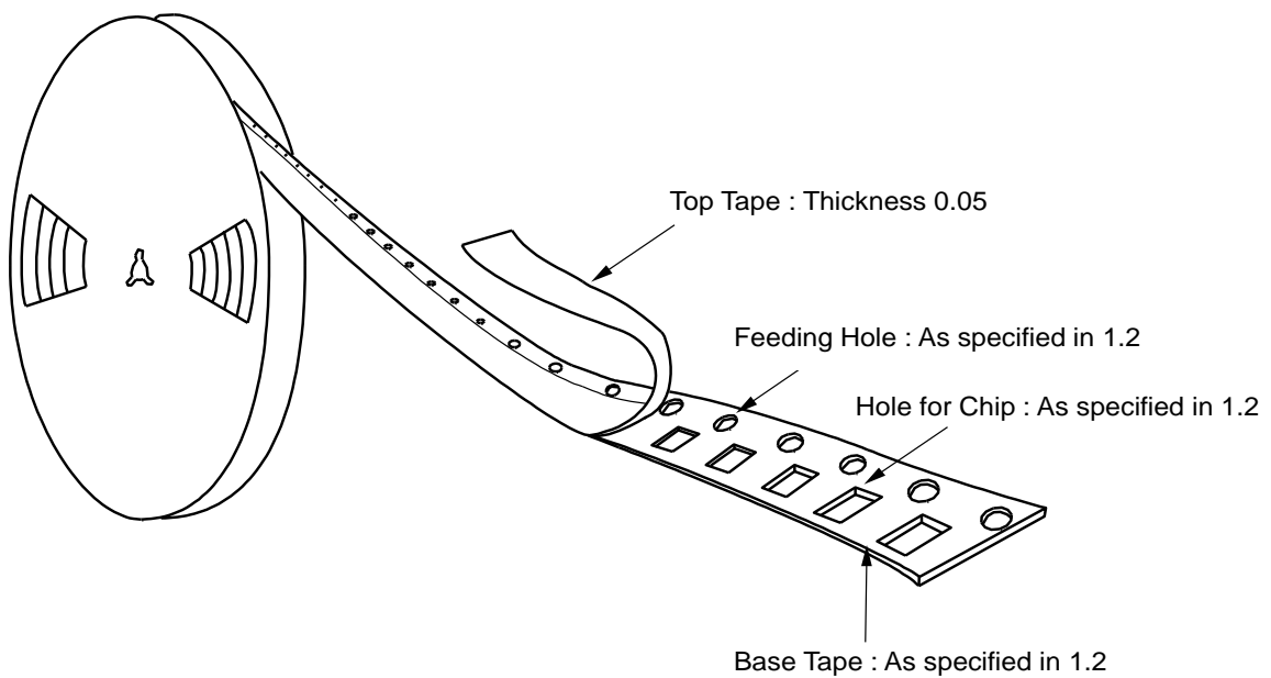
Fig3 Taping Diagram
