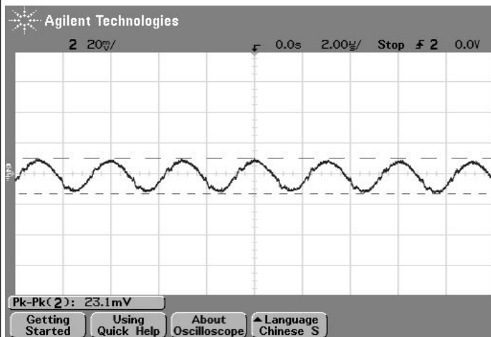
Output Ripple and noise (Vin=48V, Vout=nom., Iout=30A, Clod=0, Ta=+25° C., ScopeBW=20Mhz)
