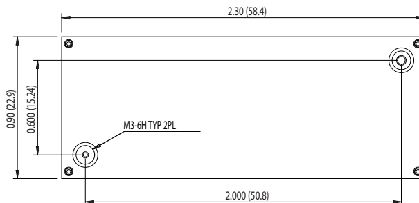
WITH BASEPLATE OPTION
