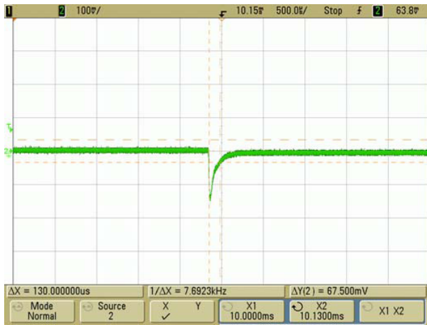
Step Load Transient Response (Slew=1A / \mu Sec., Vin=48V., Cload=0, Iout=22.5A to 15A)
