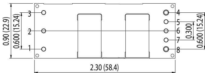
RECOMMENDED PAD LAYOUT (SMD)
