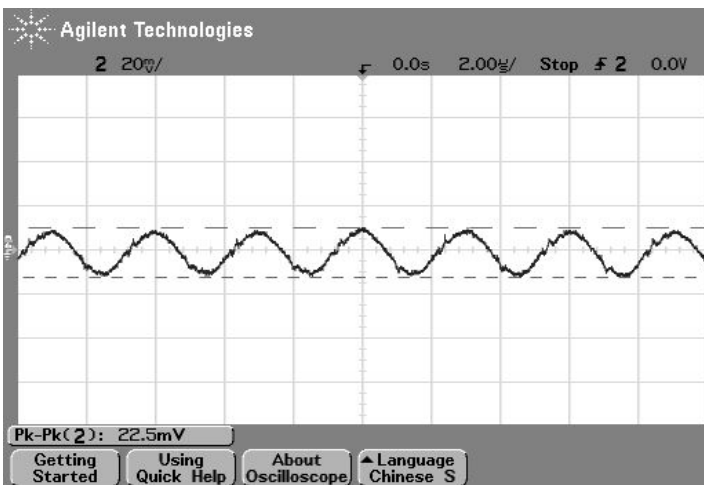
Output Ripple and noise (Vin=48V, Vout=nom., Iout=30A, Clod=0, Ta=+25° C., ScopeBW=20Mhz)
