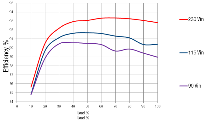
MVAC400-48 Efficiency (includes 5V Aux output)
