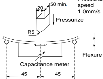
Fig.2 (in mm)
