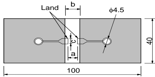
Fig.1 (in mm)
