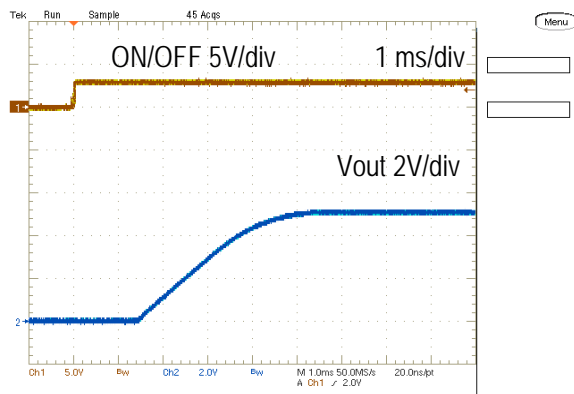
On/Off Enable Delay (Vin=12V, Vout=5.0V, Iout=4A, Cloud=400uF)
