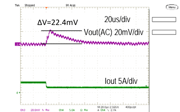
Step Load Transient Response (Vin=5.0V, Vout=1.8V, Cload=400uF, Iout=4A to 2A, 2.5A/us)
