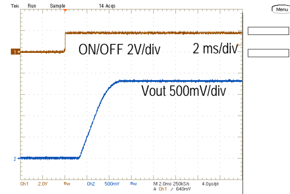
On/Off Enable Delay (Vin=5.0V, Vout=1.8V, Iout=4A, Cload=400uF)
