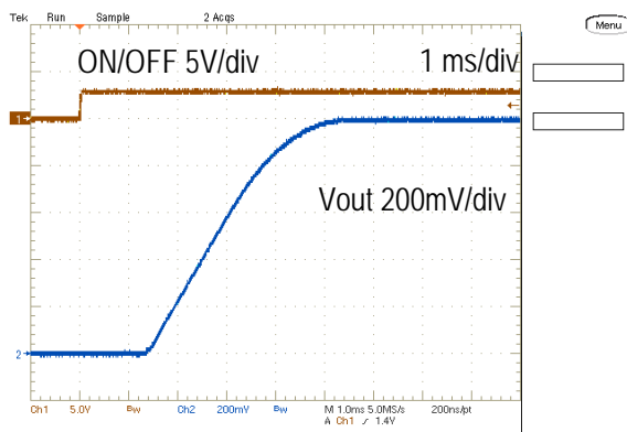
On/Off Enable Delay (Vin=12V, Vout=1.0V, Iout=4A, Cloud=400uF)
