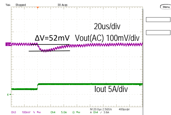
Step Load Transient Response (Vin=12V, Vout=5.0V, Cloud=400uF, Iout=2A to 4A, 2.5A/us)
