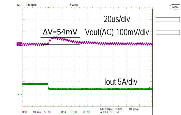
Step Load Transient Response (Vin=12V, Vout=5.0V, Cloud=400uF, Iout=4A to 2A, 2.5A/us)
