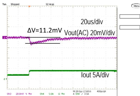
Step Load Transient Response (Vin=12V, Vout=1.0V, Cloud=400uF, Iout=2A to 4A, 2.5A/us)
