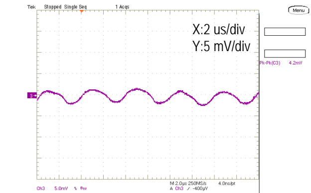
Output Ripple and Noise (Vin=5.0V, Vout=1.8V, Iout=4A, Cload=400uF, ScopeBW=20MHz)
