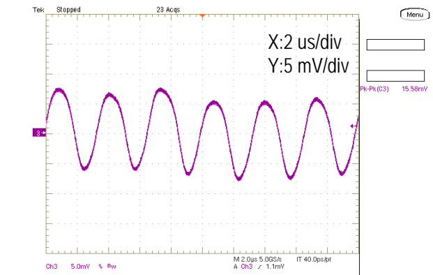
Output Ripple and Noise (Vin=12V, Vout=5.0V, Iout=4A, Cloud=400uF, ScopeBW=20MHz)
