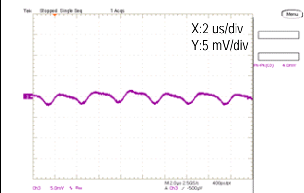
Output Ripple and Noise (Vin=12V, Vout=1.0V, Iout=4A, Cloud=400uF, ScopeBW=20MHz)
