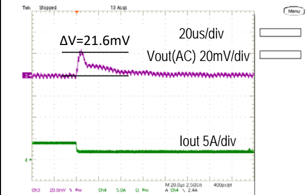
Step Load Transient Response (Vin=12V, Vout=1.0V, Cloud=400uF, Iout=4A to 2A, 2.5A/us)
