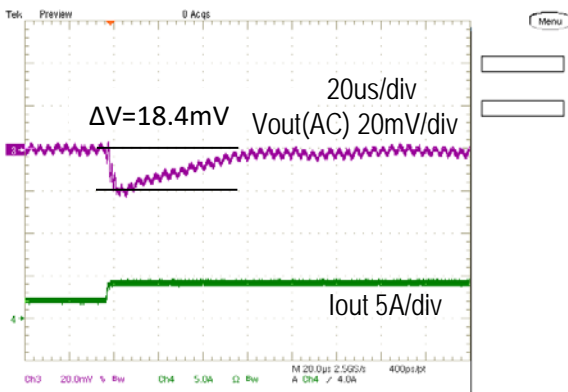
Step Load Transient Response (Vin=5.0V, Vout=1.8V, Cload=400uF, Iout=2A to 4A, 2.5A/us)
