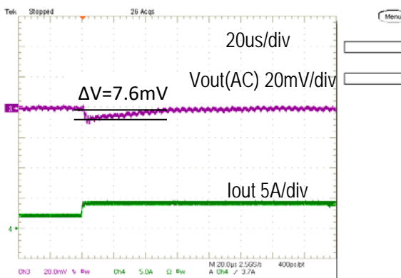
Step Load Transient Response (Vin=5.0V, Vout=0.7V, Cload=400uF, Iout=2A to 4A, 2.5A/us)
