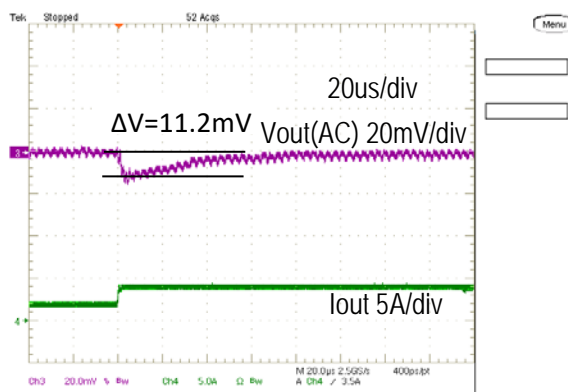
Step Load Transient Response (Vin=12V, Vout=1.0V, Cloud=400uF, Iout=2A to 4A, 2.5A/us)
