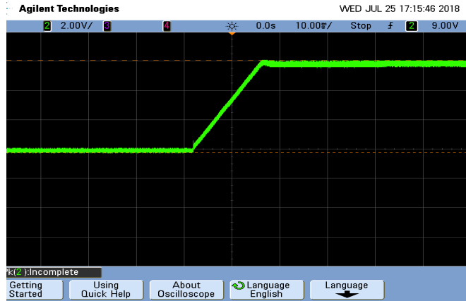
Figure 24. Output Pre-bias start-up Vin=48V, Iout = 0A, Cload = 47µF, Ta = 25°C, Pre-bias Voltage = 9.6V
