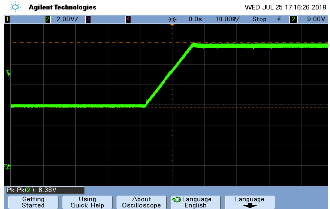
Figure 25 Output Pre-bias start-up Vin=48V, Iout = 0A, Cload = 10000µF, Ta = 25°C, Pre-bias Voltage = 9.6V
