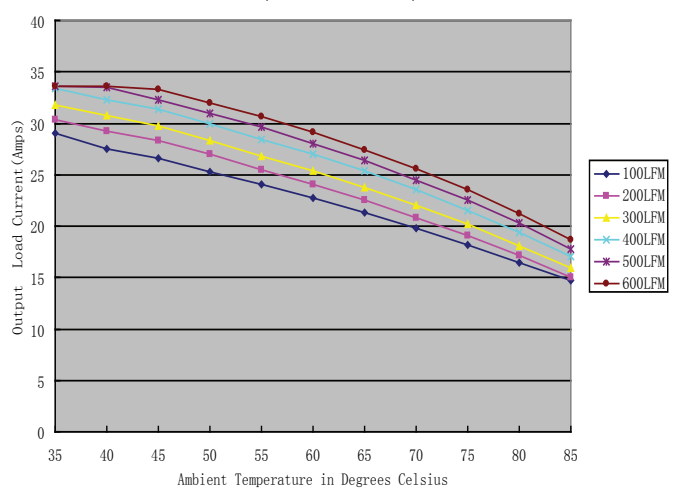
Figure 15. Temperature derating, current, longitudinal airflow vin- to vin+ 75V Input, 10" X 10" test pcb
