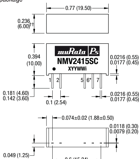
SIP package
