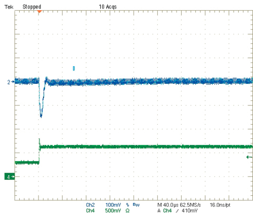
Step Load Transient Response (Vin=5V, Vout=3.3V, Clad=0, Iout=1.5A to 3A) Trace 2=Vout, 100 mV/div. Trace 4=Iout, 2.5A/div.
