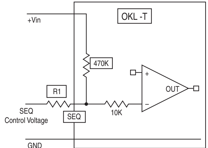
Figure 6. Sequencing Signal Interface of Module
