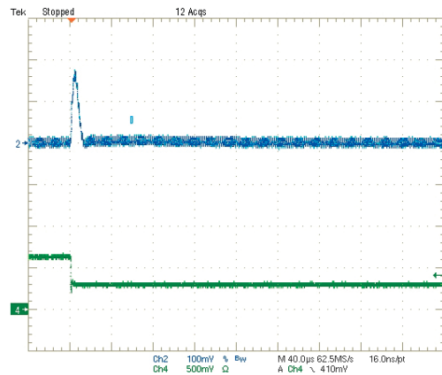
Step Load Transient Response (Vin=5V, Vout=3.3V, Clad=0, Iout=3A to 1.5A) Trace 2=Vout, 100 mV/div. Trace 4=Iout, 2.5A/div.
