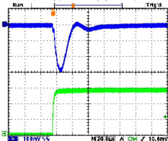
Step Load Transient Response (Vin=12V, Vout=5V, Cloud=12x10µF X5R 0805 ceramic, total 120µF, Iout=0A to 1.5A) Top trace=Vout, Bottom trace=Iout
