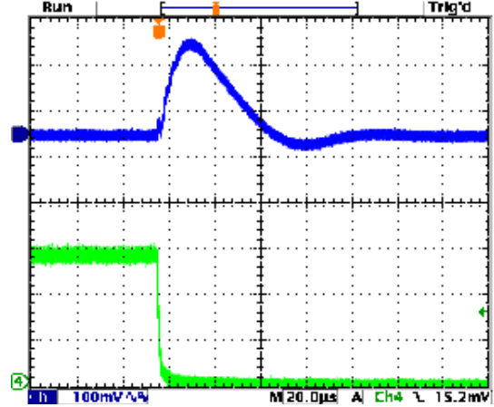
Step Load Transient Response (Vin=7.5V, Vout=5V, Cload=10x10µF X5R 0805 ceramic, plus 1x470µF, 7mΩ POSCAP, total 570µF, Iout=1.5A to 0A) Top trace=Vout, Bottom trace=Iout
