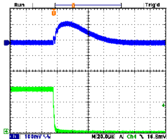
Step Load Transient Response (Vin=12V, Vout=5V, Cload=10x10µF X5R 0805 ceramic, plus 1x470µF, 7mΩ POSCAP, total 570µF, Iout=1.5A to 0A) Top trace=Vout, Bottom trace=Iout
