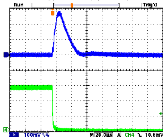
Step Load Transient Response (Vin=12V, Vout=5V, Cloud=12x10µF X5R 0805 ceramic, total 120µF, Iout=1.5A to 0A) Top trace=Vout, Bottom trace=Iout
