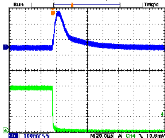
Step Load Transient Response (Vin=7.5V, Vout=5V, Cloud=5x10µF X5R 0805 ceramic, total 50µF, Iout=1.5A to 0A) Top trace=Vout, Bottom trace=Iout
