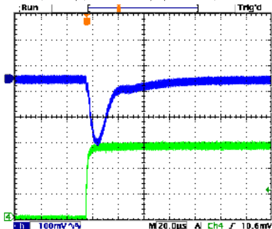
Step Load Transient Response (Vin=7.5V, Vout=5V, Cloud=5x10µF X5R 0805 ceramic, total 50µF, Iout=0A to 1.5A) Top trace=Vout, Bottom trace=Iout
