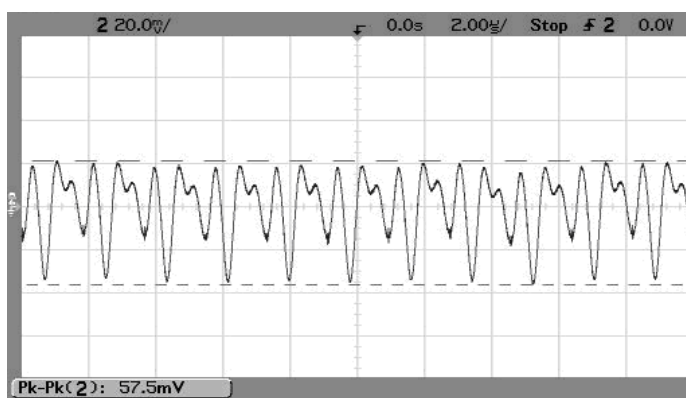
Step Load Transient Response (Vin=12V, Vout=2.5V, Load=0, Iout=6A to 3A)
