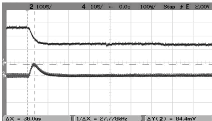
Step Load Transient Response (Vin=5V, Vout=1.2V, Cload=0, Iout=5A to 2.5A) Trace 2=Vout, 100 mV/div. Trace 4=Iout, 2A/div.
