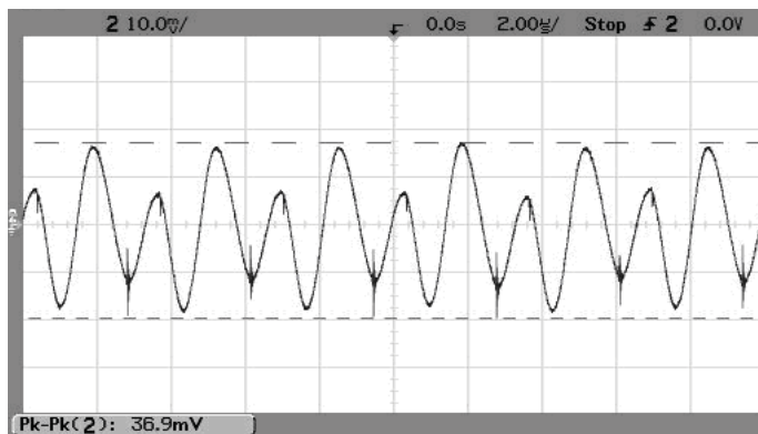
Output Ripple and Noise (Vin=5V, Vout=1.2V, Iout=5A, Cload=0, ScopeBW=100MHz)
