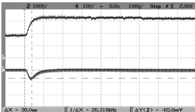
Step Load Transient Response (Vin=5V, Vout=2.5V, Load=0, Iout=1.5A to 3A) Trace 2=Vout, 100 mV/div. Trace 4=Iout, 1A/div.
