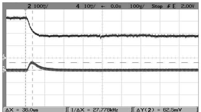
Step Load Transient Response (Vin=5V, Vout=2.5V, Load=0, Iout=3A to 1.5A) Trace 2=Vout, 100 mV/div. Trace 4=Iout, 1A/div.
