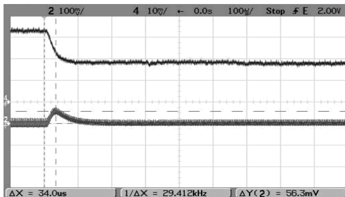
Step Load Transient Response (Vin=5V, Vout=1.2V, Clod=0, Iout=3A to 1.5A) Trace 2=Vout, 100 mV/div. Trace 4=Iout, 1A/div.
