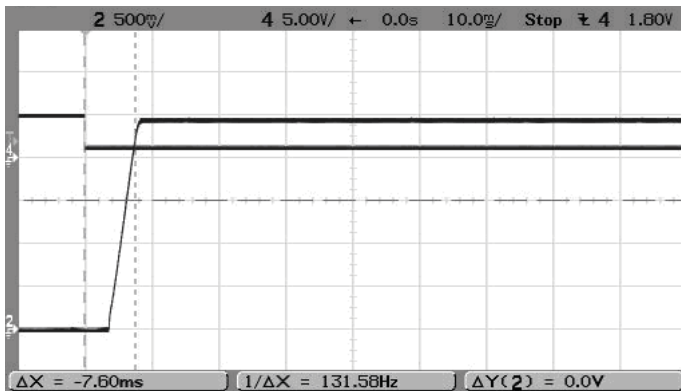
On/Off Enable Startup (Vin=5.5V, Vout=2.5V, Iout=3A, Load=0) Trace 4=Enable, Trace 2=Vout
