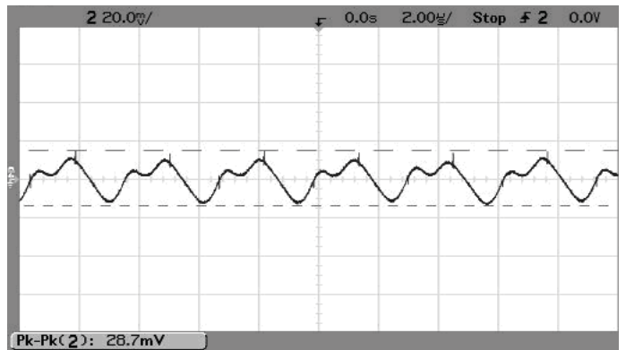
Output Ripple and Noise (Vin=5V, Vout=2.5V, Iout=3A, Load=0, ScopeBW=100MHz)
