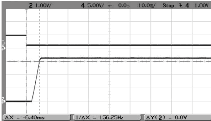
On/Off Enable Startup (Vin=5.5V, Vout=3.3V, Iout=5A, Load=0) Trace 4=Enable, Trace 2=Vout
