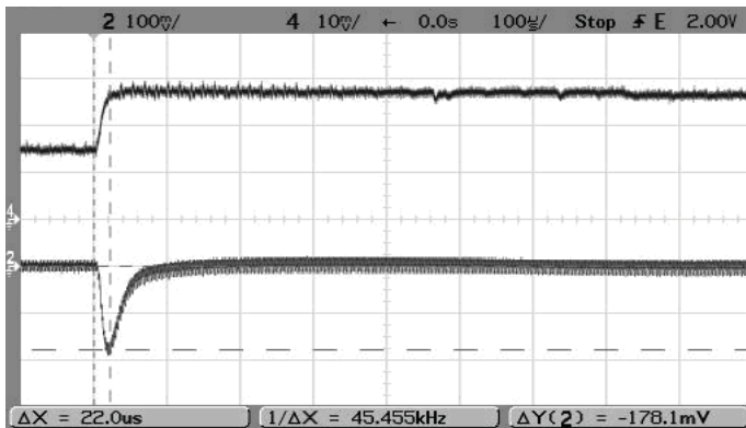
Step Load Transient Response (Vin=5V, Vout=3.3V, Load=0, Iout=2.5A to 5A) Trace 2=Vout, 100 mV/div. Trace 4=Iout, 2A/div.
