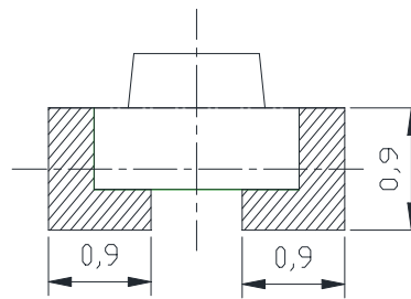
推荐焊盘尺寸 Recommended Soldering Pad
