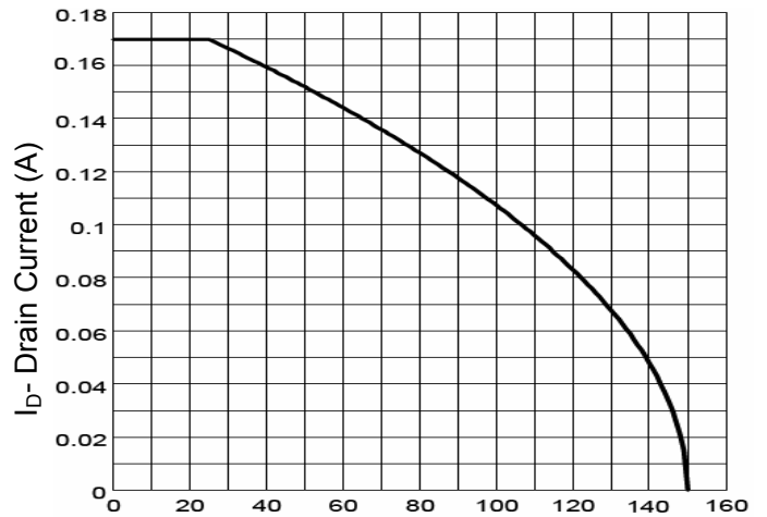
T_J -Junction Temperature( ^{\circ}\text{C} ) Figure 10 Current De-rating
