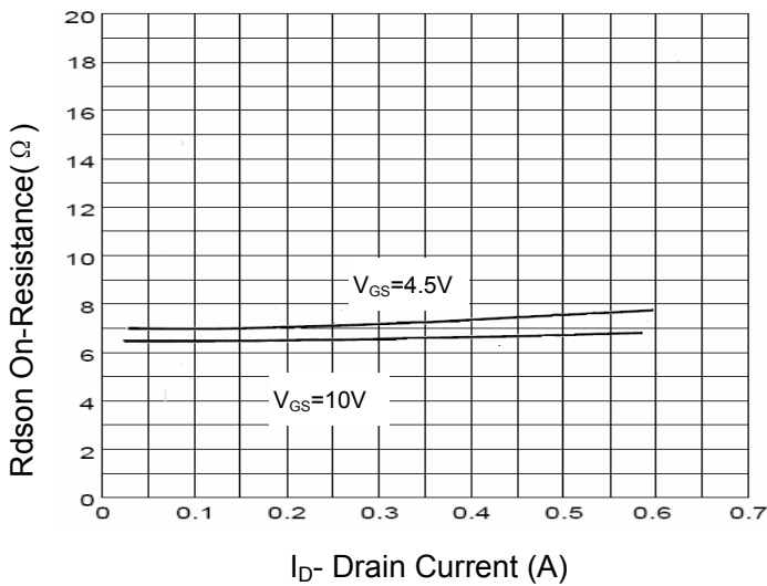
Figure 5 Drain-Source On-Resistance
