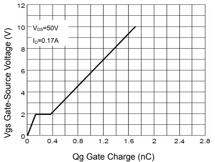
Figure 6 Gate Charge
