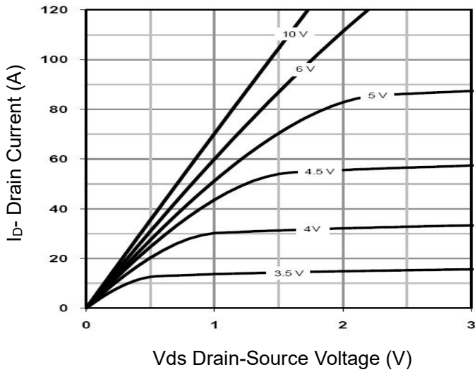
Figure 1 Output Characteristics
