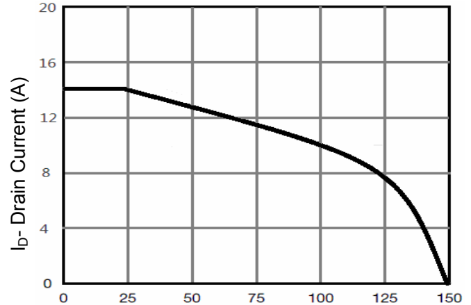
Figure 10 Current De-rating
