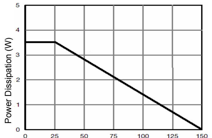
Figure 9 Power De-rating
