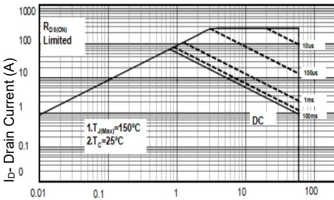
Figure 8 Safe Operation Area
