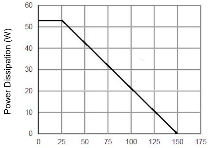
Figure 9 Power De-rating
