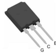
TO-247P
