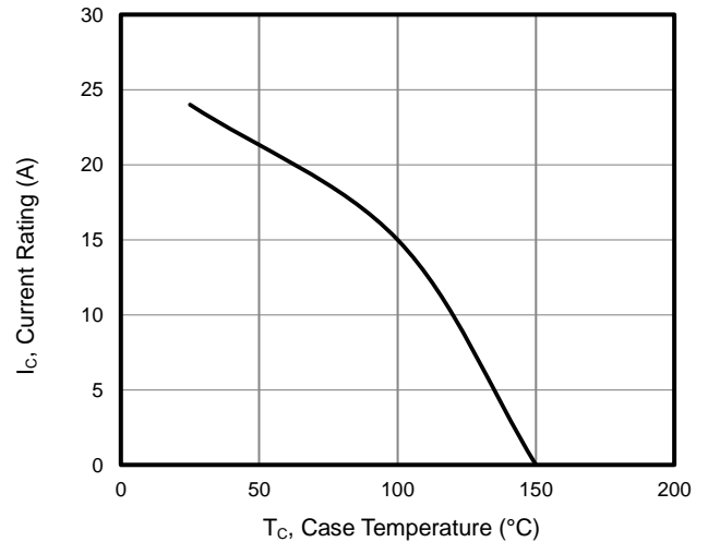
Figure 12 Current De-rating
