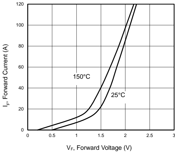
Figure 13 Forward Characteristics
