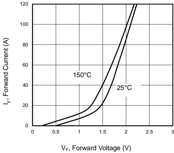
Figure 7 Forward Characteristics
