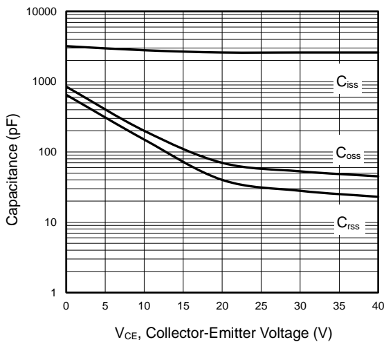
Figure 5 Capacitance Characteristics
