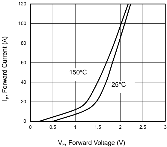
Figure 7 Forward Characteristics
