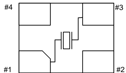
TERMINAL #1,#3:X'tal #2,#4:GND(CONNECTION COVER)
