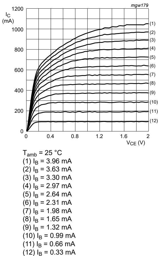
Fig. 5. Collector current as a function of collector-emitter voltage; typical values
