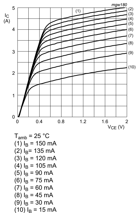
Fig. 6. Collector current as a function of collector-emitter voltage; typical values.
