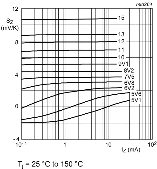
Fig. 3. Temperature coefficient as a function of working current; typical values (BZB784-C5V1 to C15)
