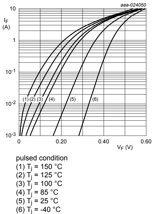
Fig. 3. Forward current as a function of forward voltage; typical values
