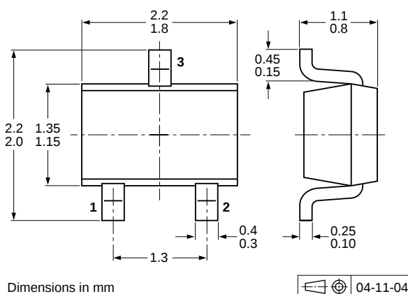
Fig 15. Package outline PDTA143EU (SOT323/SC-70)
