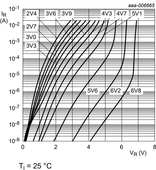
Fig. 8. Reverse current as a function of reverse voltage; typical values (BZX585-B/C2V4 to BZX585-B/C6V8)
