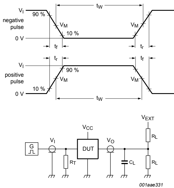
Test data is given in Table 9 . All input pulses are supplied by generators having the following characteristics: PRR \leq 10 \text{ MHz} ; Z_o = 50 \, \Omega . The outputs are measured one at a time with one transition per measurement. Definitions for test circuit: R_L = Load resistance. C_L = Load capacitance including jig and probe capacitance. R_T = Termination resistance should be equal to output impedance Z_o of the pulse generator. V_{EXT} = External voltage for measuring switching times.
