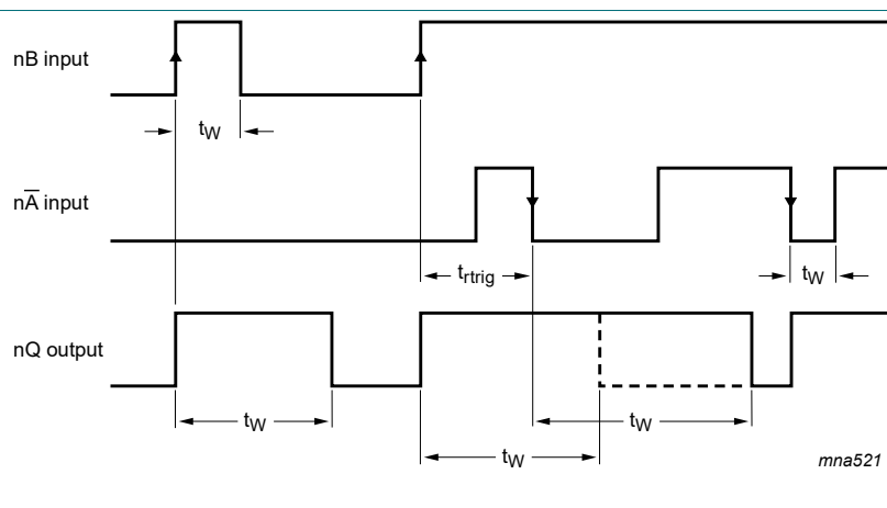
Fig. 8. Output pulse control using retrigger pulse
