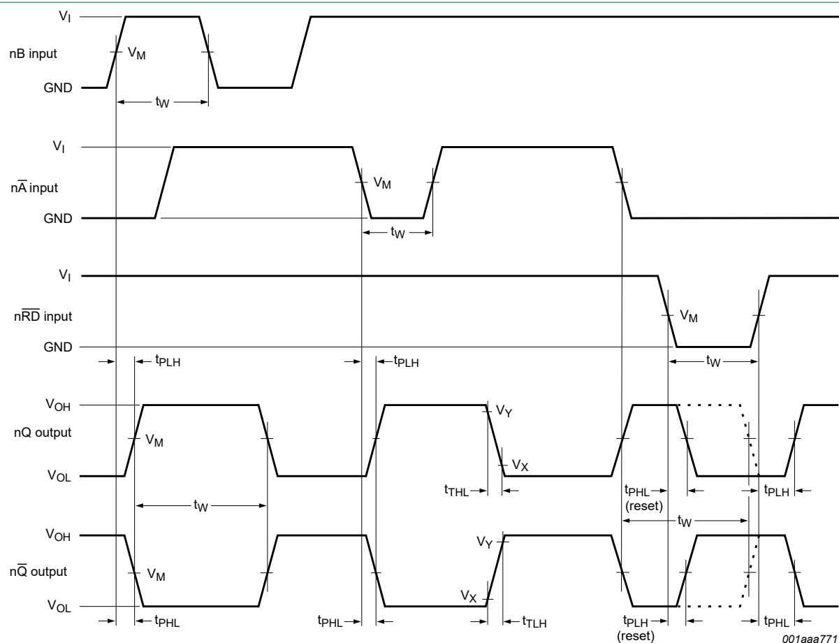
Fig. 7. Propagation delays from inputs ( n\bar{A} , nB , n\bar{RD} ) to outputs ( nQ , n\bar{Q} ) and output transition times
