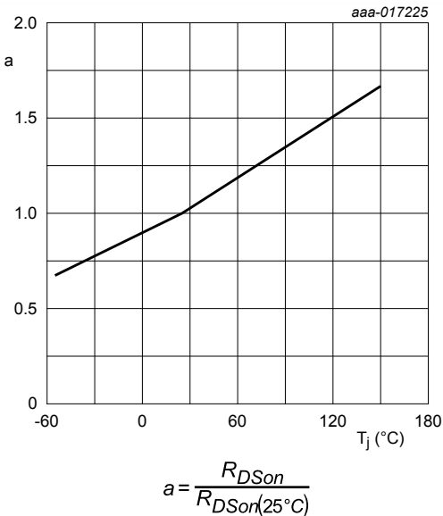
Fig. 24. TR2: Normalized drain-source on-state resistance as a function of ambient temperature; typical values
