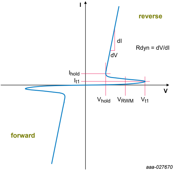
Fig. 9. V-I characteristics for a bidirectional ESD protection diode
