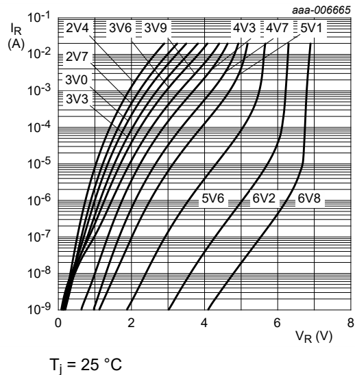
Fig. 8. Reverse current as a function of reverse voltage; typical values (BZX84-A/B/C2V4-Q to BZX84-A/B/C6V8-Q)
