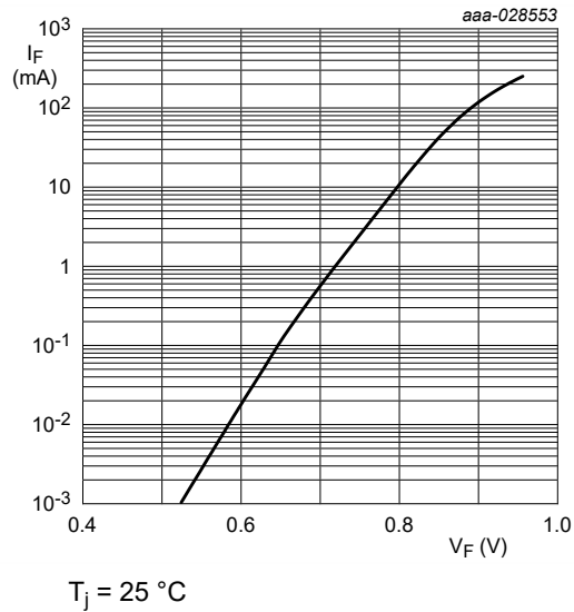
Fig. 5. Forward current as a function of forward voltage; typical values (BZX84-A/B/C75-Q)
