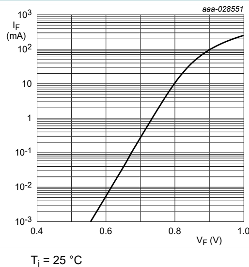
Fig. 3. Forward current as a function of forward voltage; typical values (BZX84-A/B/C6V8-Q)
