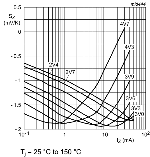
Fig. 6. Temperature coefficient as a function of working current; typical values (BZX84-A/B/C2V4-Q to BZX84-A/B/C4V7-Q)
