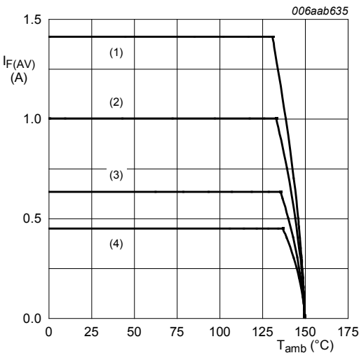
Ceramic PCB, \text{Al}_2\text{O}_3 , standard footprint T_j = 150 °C (1) \delta = 1 ; DC (2) \delta = 0.5 ; f = 20 kHz (3) \delta = 0.2 ; f = 20 kHz (4) \delta = 0.1 ; f = 20 kHz
