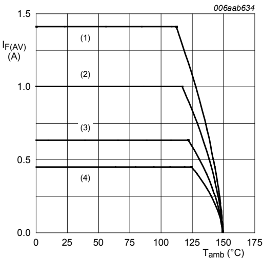
FR4 PCB, mounting pad for cathode 1\text{ cm}^2 T_j = 150 °C (1) \delta = 1 ; DC (2) \delta = 0.5 ; f = 20 kHz (3) \delta = 0.2 ; f = 20 kHz (4) \delta = 0.1 ; f = 20 kHz
