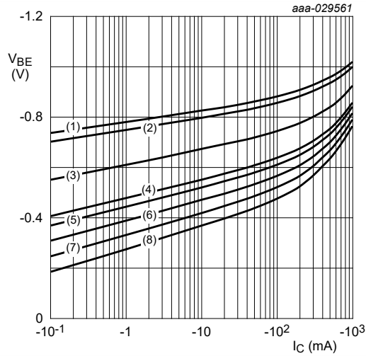
V_{CE} = -1\text{ V} (1) T_{amb} = -55\text{ }^{\circ}\text{C} (2) T_{amb} = -40\text{ }^{\circ}\text{C} (3) T_{amb} = 25\text{ }^{\circ}\text{C} (4) T_{amb} = 85\text{ }^{\circ}\text{C} (5) T_{amb} = 100\text{ }^{\circ}\text{C} (6) T_{amb} = 125\text{ }^{\circ}\text{C} (7) T_{amb} = 150\text{ }^{\circ}\text{C} (8) T_{amb} = 175\text{ }^{\circ}\text{C}
