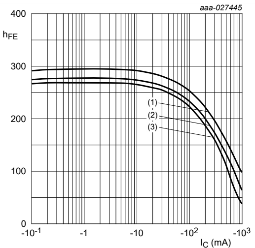
T_{amb} = 25\text{ }^{\circ}\text{C} (1) V_{CE} = -5\text{ V} (2) V_{CE} = -2\text{ V} (3) V_{CE} = -1\text{ V}
