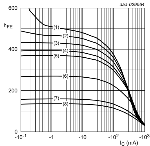
V_{CE} = -1\text{ V} (1) T_{amb} = 175\text{ }^{\circ}\text{C} (2) T_{amb} = 150\text{ }^{\circ}\text{C} (3) T_{amb} = 125\text{ }^{\circ}\text{C} (4) T_{amb} = 100\text{ }^{\circ}\text{C} (5) T_{amb} = 85\text{ }^{\circ}\text{C} (6) T_{amb} = 25\text{ }^{\circ}\text{C} (7) T_{amb} = -40\text{ }^{\circ}\text{C} (8) T_{amb} = -55\text{ }^{\circ}\text{C}
