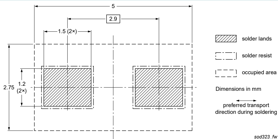
Fig. 9. Wave soldering footprint for SOD323
