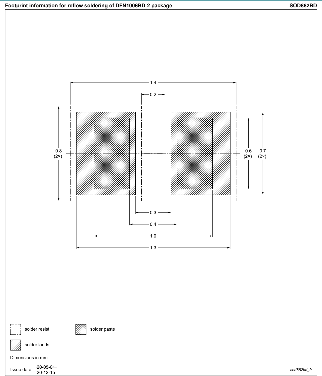
Fig. 11. Reflow soldering footprint for DFN1006BD-2 (SOD882BD)
