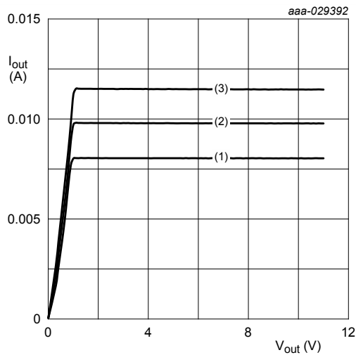
V_{EN} = 12\text{ V} ; R_{ext} = \text{open} (1) T_{amb} = 85\text{ °C} (2) T_{amb} = 25\text{ °C} (3) T_{amb} = -40\text{ °C}
