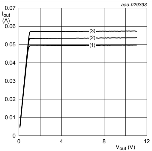
V_{EN} = 12\text{ V} ; R_{ext} = 20\text{ }\Omega (1) T_{amb} = 85\text{ °C} (2) T_{amb} = 25\text{ °C} (3) T_{amb} = -40\text{ °C}
