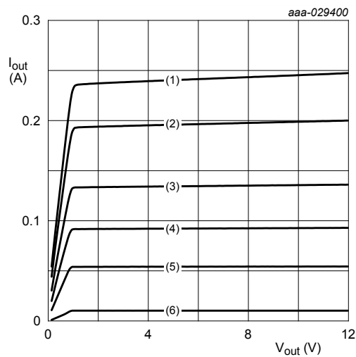
V_{EN} = 3.3\text{ V} ; T_{amb} = 25\text{ }^{\circ}\text{C} (1) R_{ext} = 3\text{ }\Omega (2) R_{ext} = 4\text{ }\Omega (3) R_{ext} = 6\text{ }\Omega (4) R_{ext} = 10\text{ }\Omega (5) R_{ext} = 20\text{ }\Omega (6) R_{ext} = \text{open}
