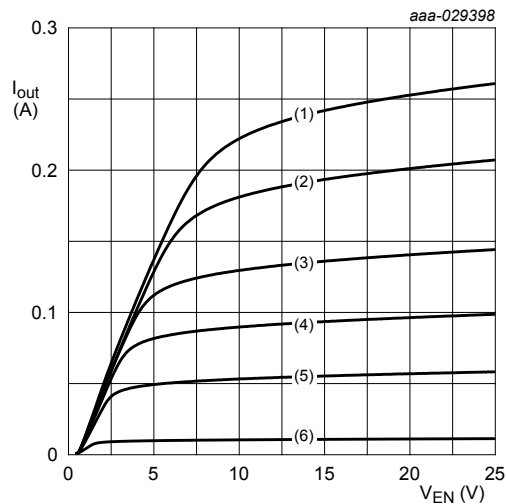
V_{out} = 2\text{ V} ; T_{amb} = 25\text{ }^{\circ}\text{C} (1) R_{ext} = 3\text{ }\Omega (2) R_{ext} = 4\text{ }\Omega (3) R_{ext} = 6\text{ }\Omega (4) R_{ext} = 10\text{ }\Omega (5) R_{ext} = 20\text{ }\Omega (6) R_{ext} = \text{open}
