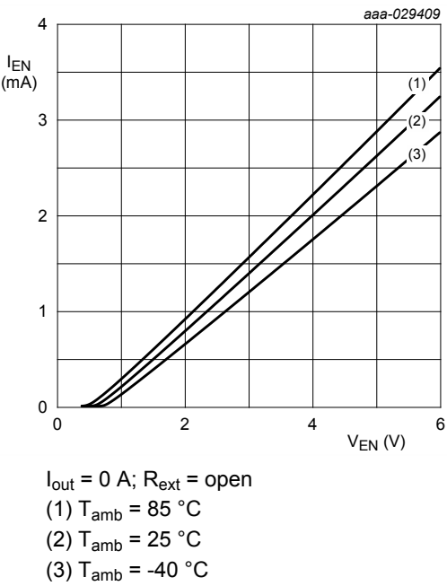
Fig. 23. NCR321U: Enable current as a function of enable voltage; typical values
