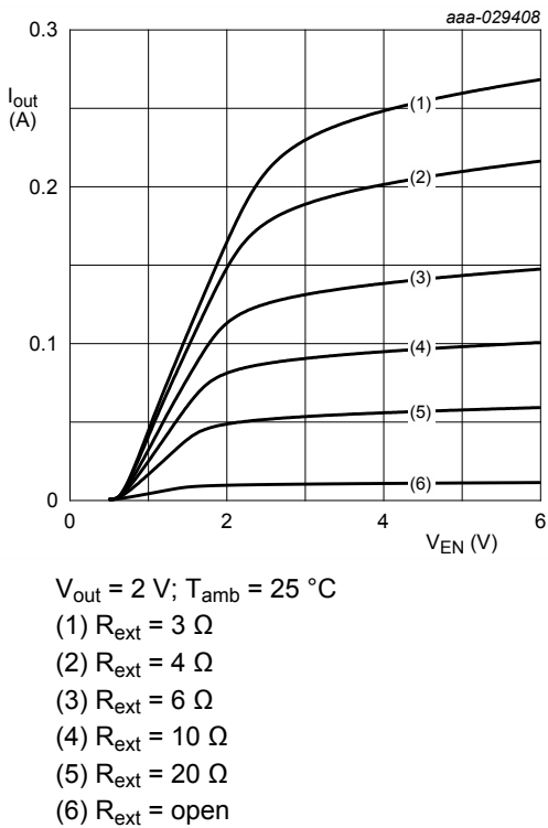
Fig. 22. NCR321U: Output current as a function of enable voltage; typical values
