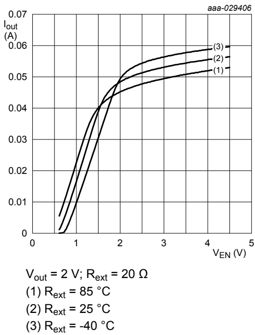
Fig. 20. NCR321U: Output current as a function of enable voltage; typical values
