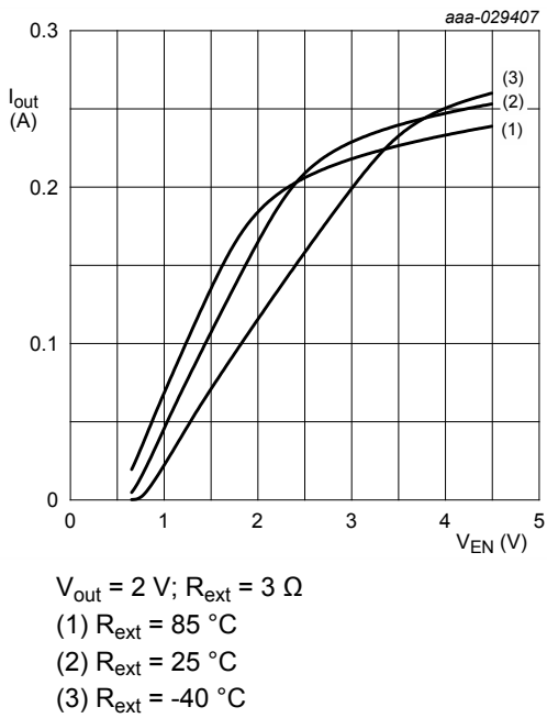
Fig. 21. NCR321U: Output current as a function of enable voltage; typical values
