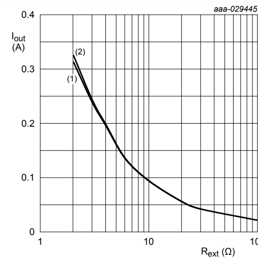
V_{EN} = 3.3\text{ V} ; T_{amb} = 25\text{ }^{\circ}\text{C} (1) V_{out} = 1.4\text{ V} (2) V_{out} = 5.4\text{ V}
